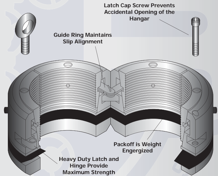
BB-22 Casing Hanger
