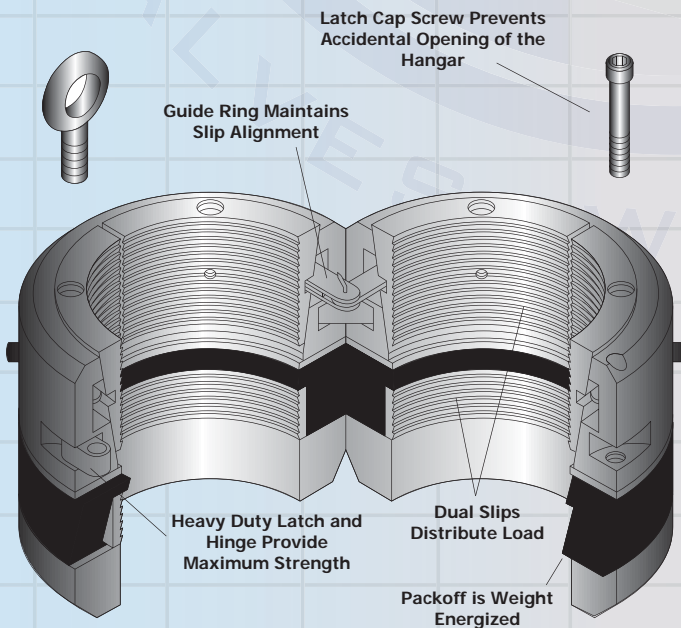
BB-29 Casing Hanger
