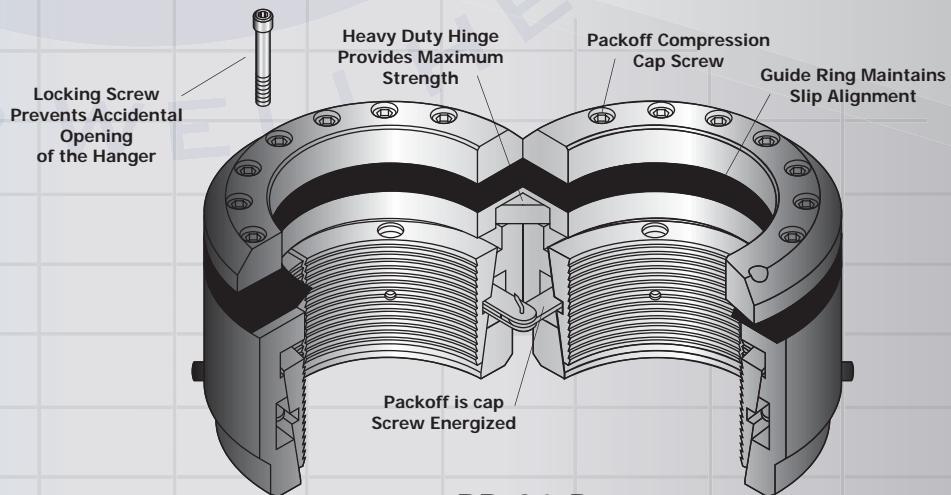
BB-21-P Casing Hanger
