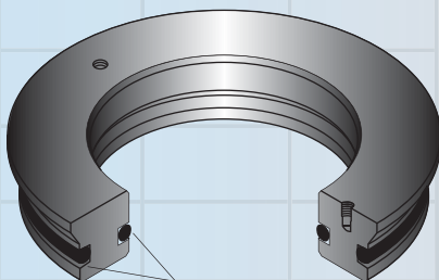
Self Energized O-Ring Protects Ring Gasket and Slips from Annular Pressure
